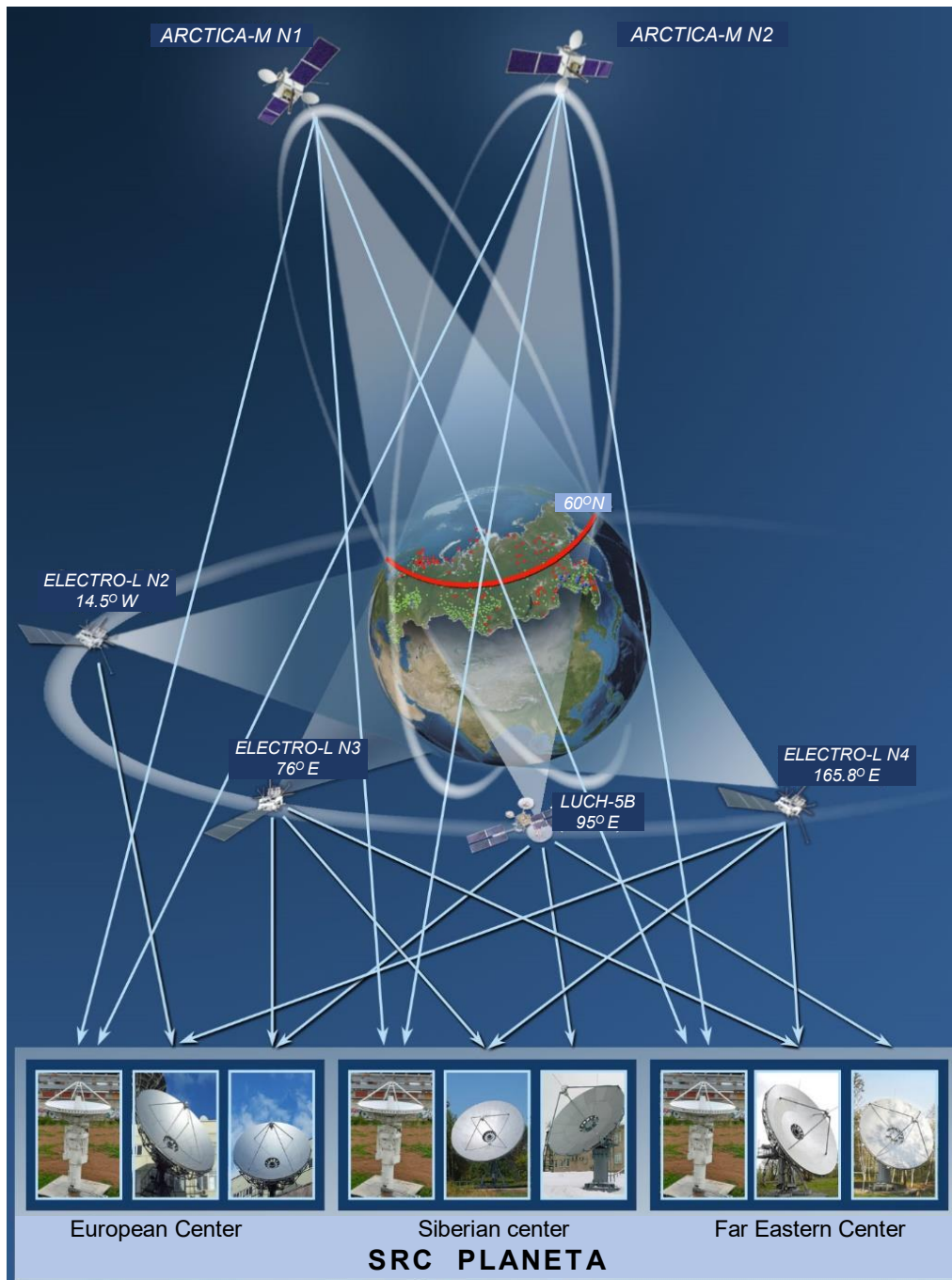
Figure 2: Russian DCS functional diagram.
