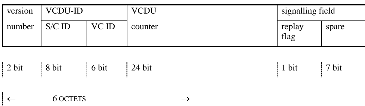
Figure 8-5 VCDU Primary Header
