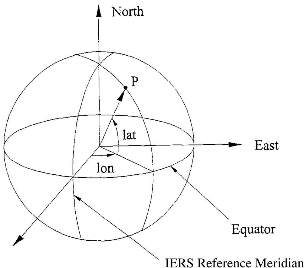
Figure 4-6 Geographical Coordinates
