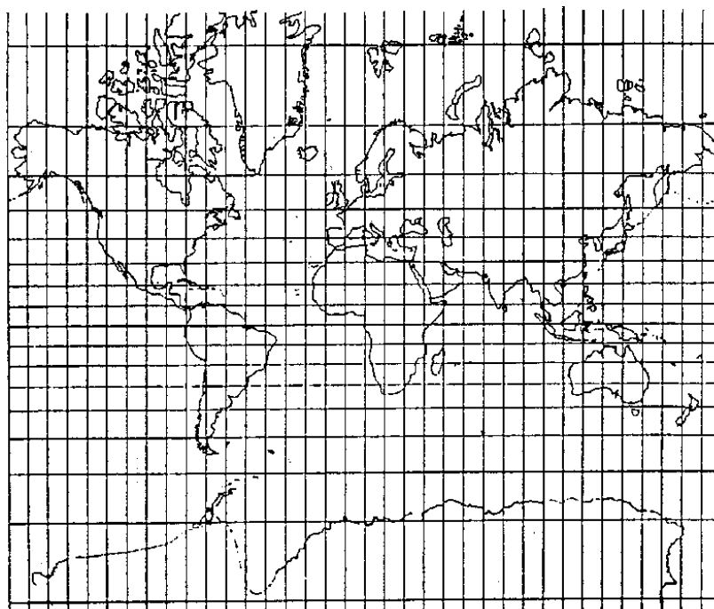
Figure 4-10 Mercator Projection
