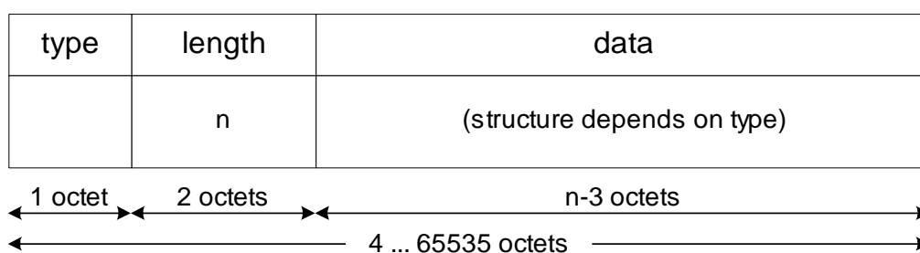
Figure 4-2 General LRIT/HRIT Header Record Structure
