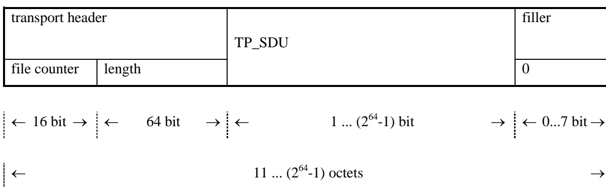
Figure 6-1 Transport File Structure
