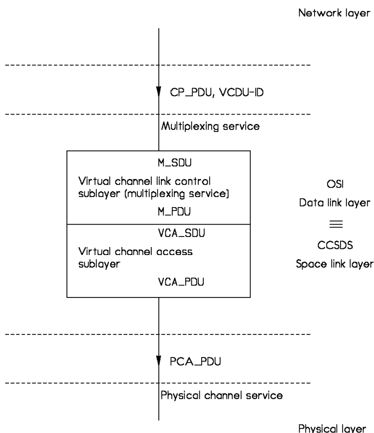
Figure 8-1 Data Link Layer
